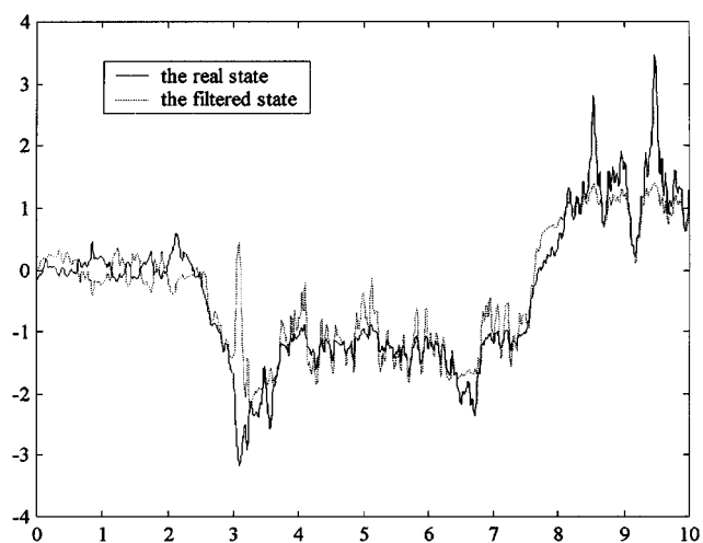
Fig. 2. The true and estimated states: first component.
